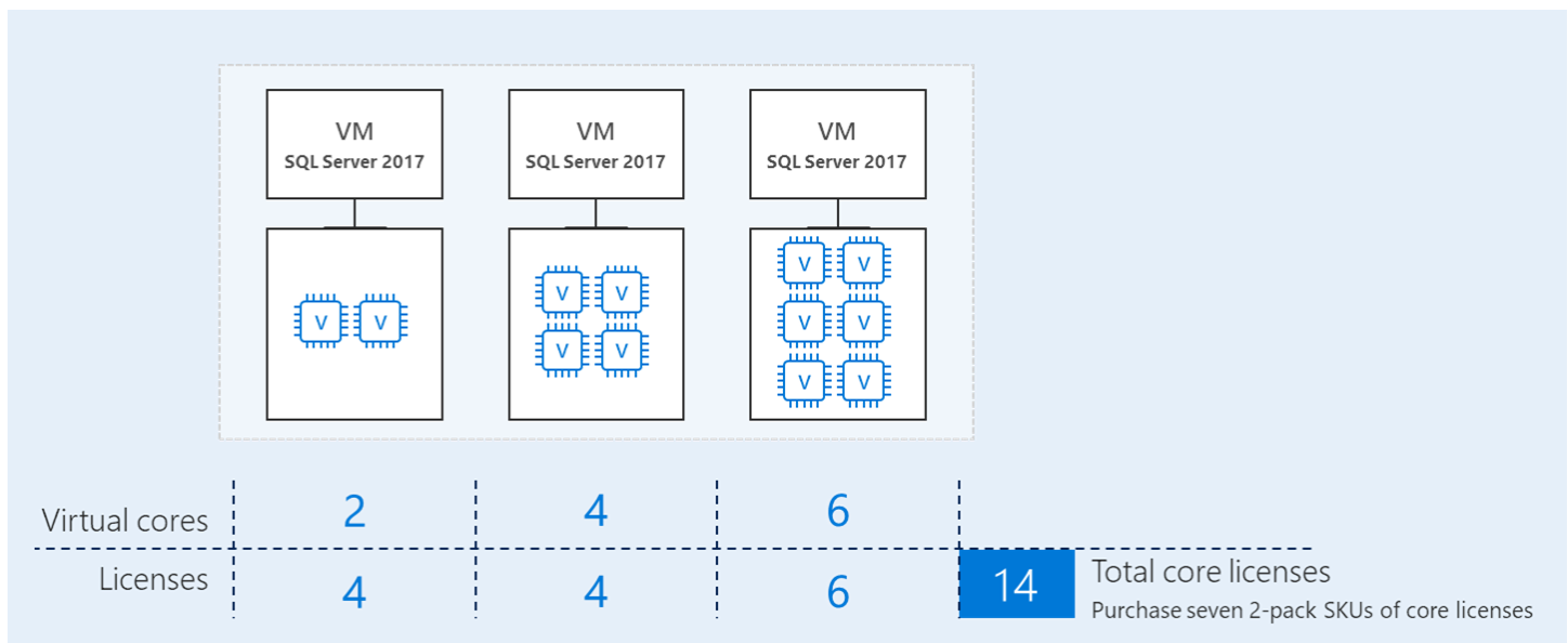
This figure illustrates the licensing requirements for three different virtual machines under the Per Core licensing model.
